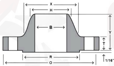
WELD NECK
